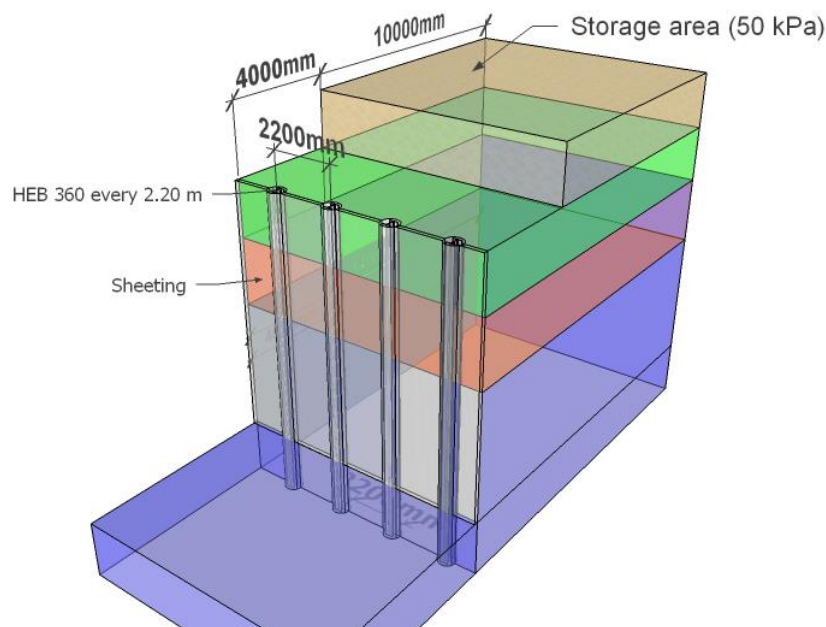
3D view of retaining structure project
