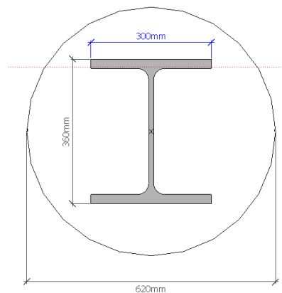
Plan view of a 620 mm pile reinforced with an HEB360 section
