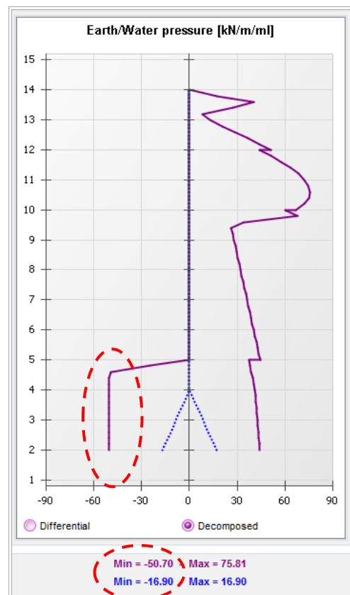
Pressure profile after reduction of p_{\max}
