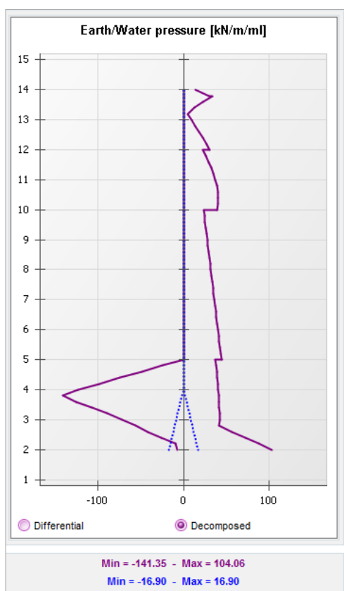
Pressure profile before reduction of p_{\max}
