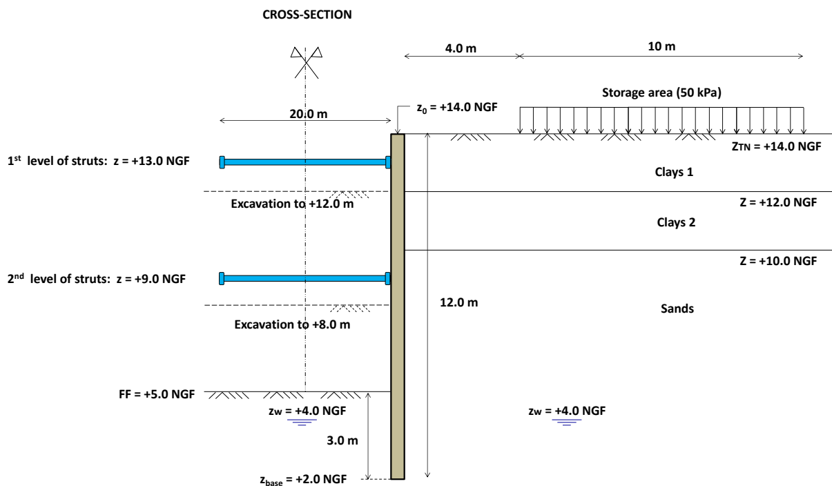
Calculation cross-section
