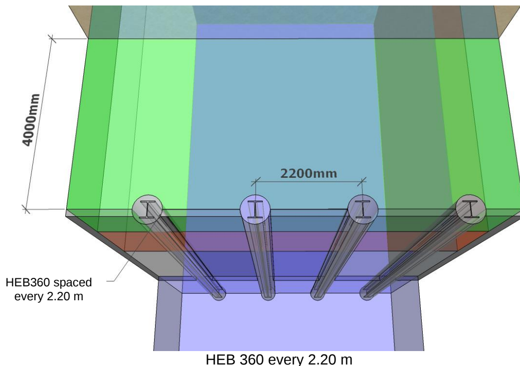
Plan view of retaining structure from excavation side
